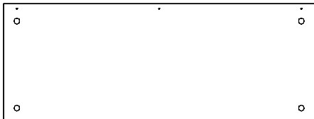
B Bottom (1) 31-1/2" x 11-3/4" 023202Z
