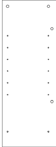
C Right Side (1) 31-1/2" x 11-3/4" 033201Z
